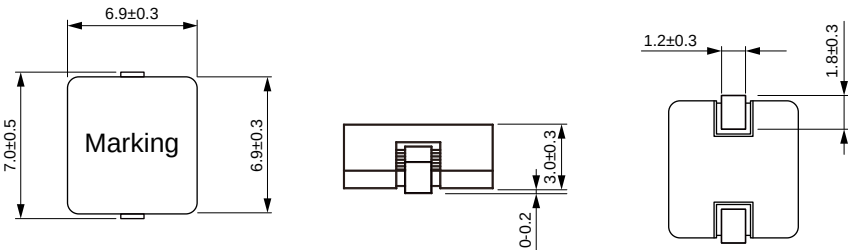
Dimensions: [mm]
